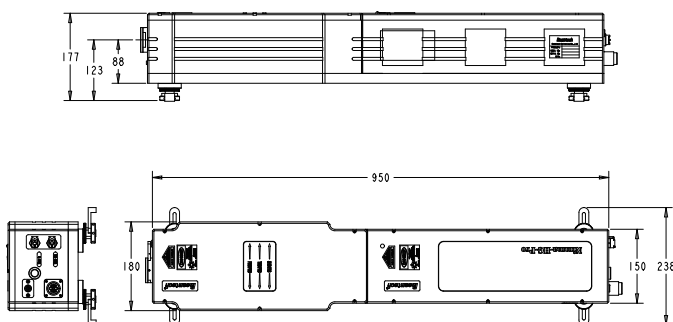
Nimma-HG-Pro-400/600/900 Laser head
