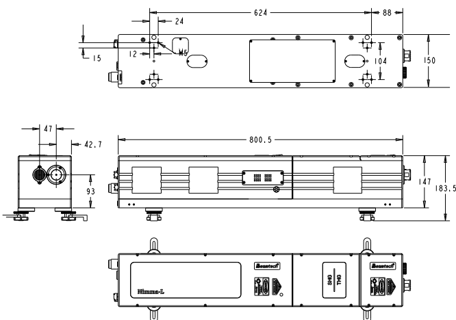
Laser head
